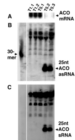
Twenty-five-nucleotide ACO antisense and sense RNA in PTGS lines
